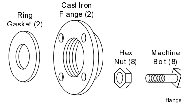
Companion Flange and Gasket
